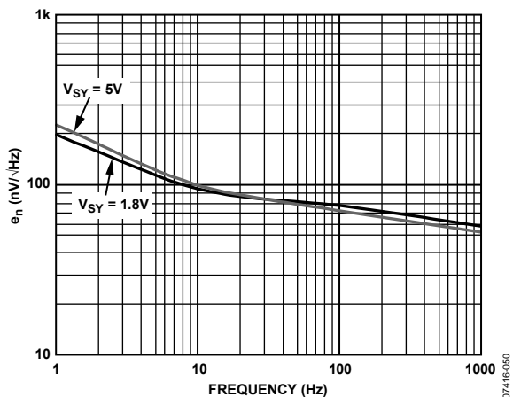
Figure 31. Voltage Noise Density vs. Frequency
